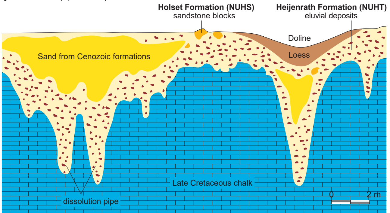
Schematic cross section at the location of the Vylenerbos (South-Limburg) with the stratigraphic positions of the Holset and Heijenrath formations.
