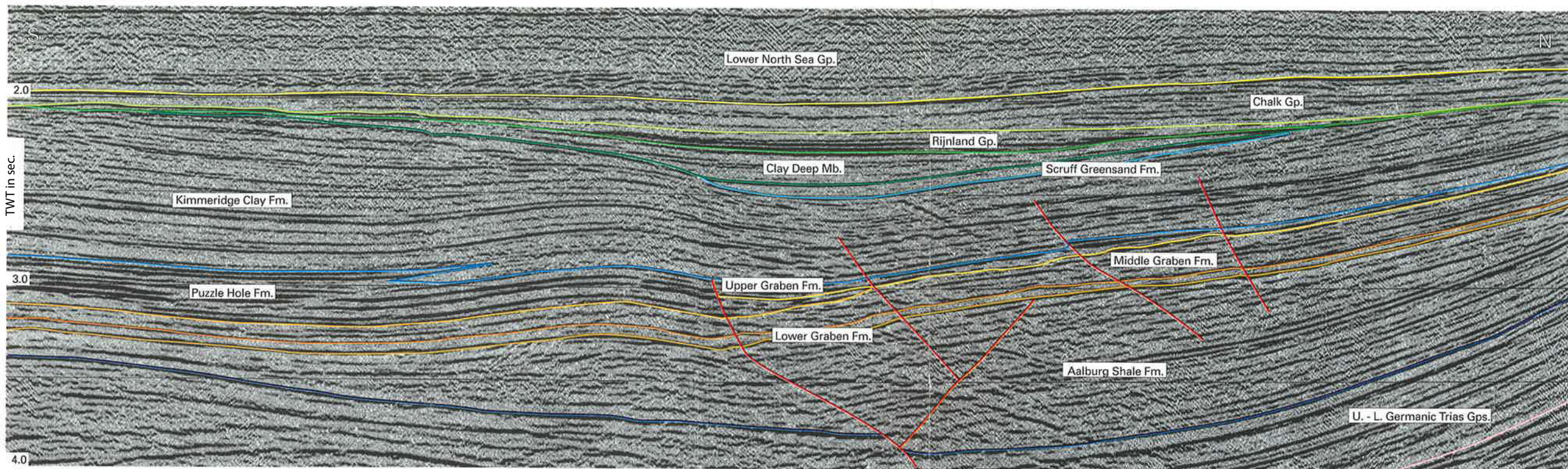
Fig.G.9 Example of Upper Jurassic-Lower Cretaceous seismic facies in the northern-central parts of the Dutch Central Graben. Line runs roughly N-S, though offshore blocks F05 and F08 (courtesy of HGS Ltd.). Note the northward transition of the Puzzle Hole Fm. into the Upper Graben Fm.
