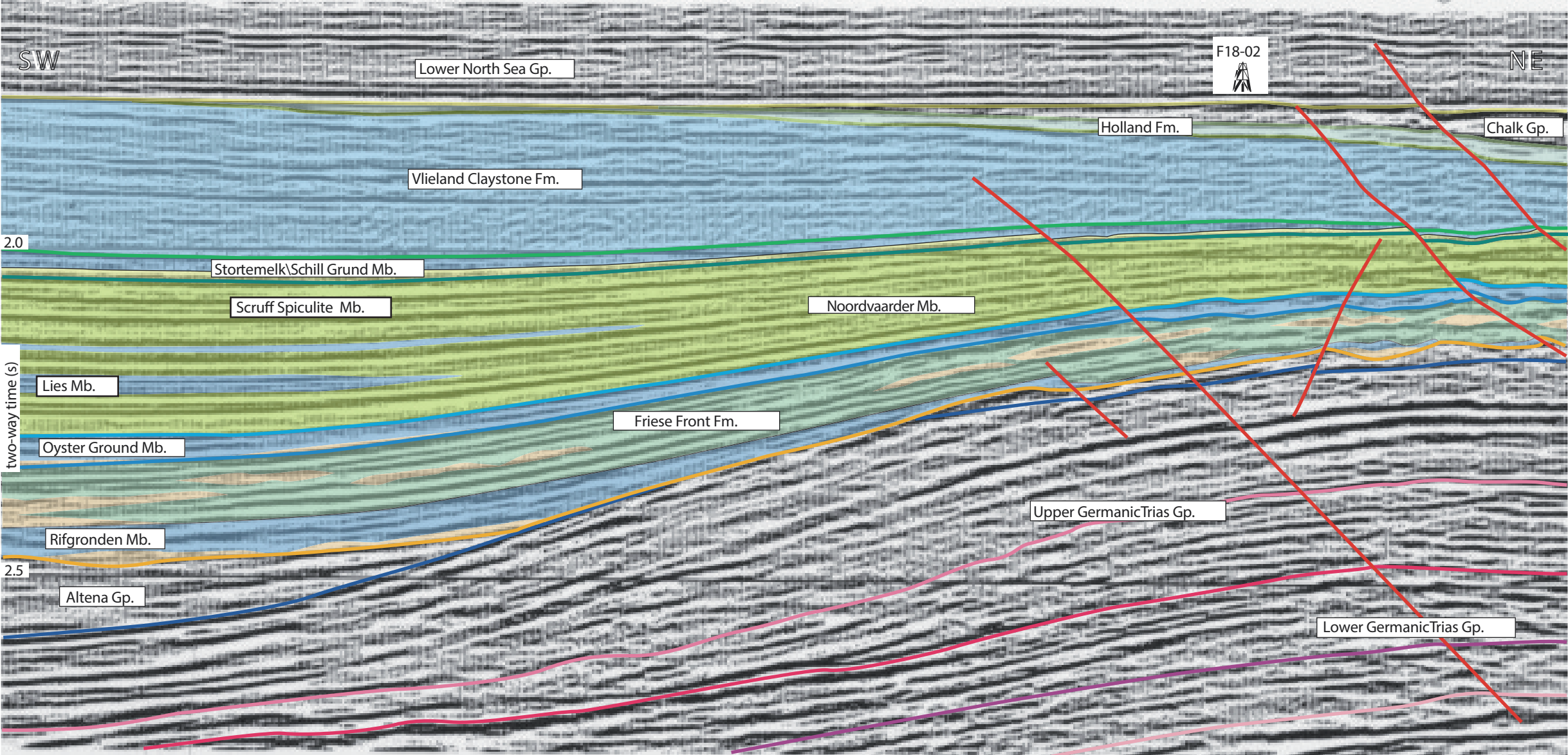
Figure G.10 Example of Upper Jurassic - Lower Cretaceous seismic facies in the western Terschelling Basin. Lines runs roughly N
